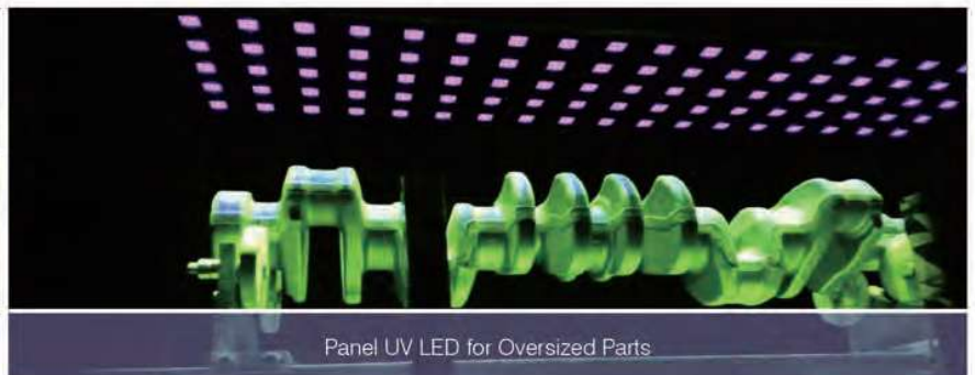
Special Panel UV LED for FPI Rinsing Station
